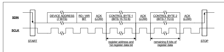
Figure 26 2-Wire Serial Control Interface
