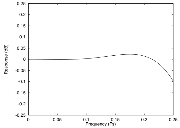
Figure 42 ADC Digital Filter Ripple – Type 3
