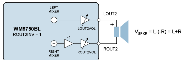
Figure 14 Speaker Output Connection
