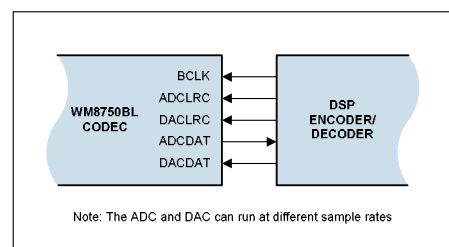
Figure 17 Slave Mode
