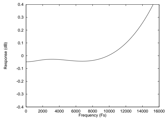
Figure 44 De-emphasis Error (32kHz)
