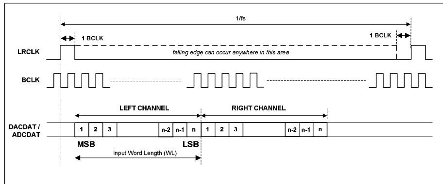
Figure 22 DSP/PCM Mode Audio Interface (mode A, LRP=0, Slave)
