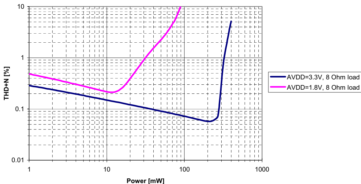
Speaker Output Power vs THD+N
