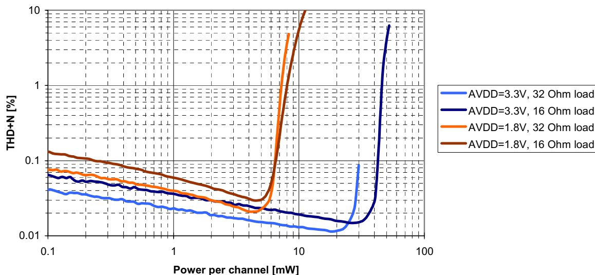
Headphone Output Power vs THD+N
