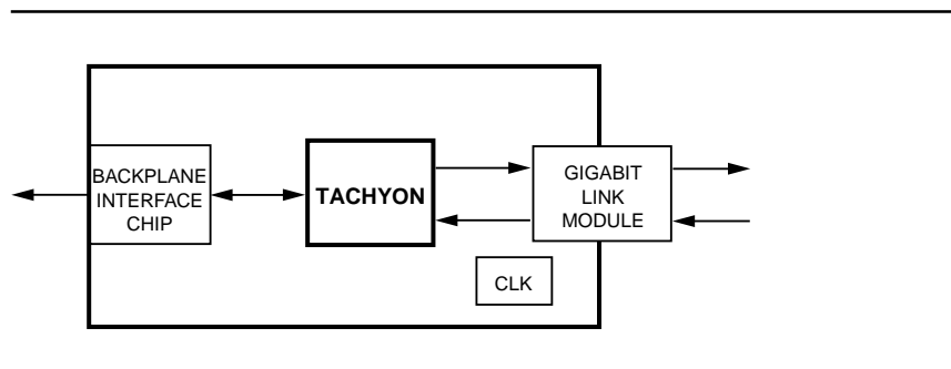
Figure 2. System Adapter Card Block Diagram
