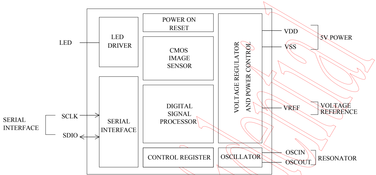
Figure 3. Block diagram
