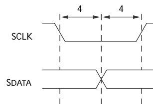
Figure 37: Serial Host Interface Write Data Timing
