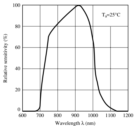
Fig.12 Spectral Sensitivity
