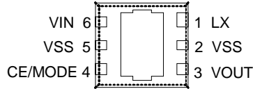
USP-6B (BOTTOM VIEW)
