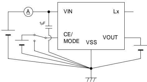
Circuit ⑤
